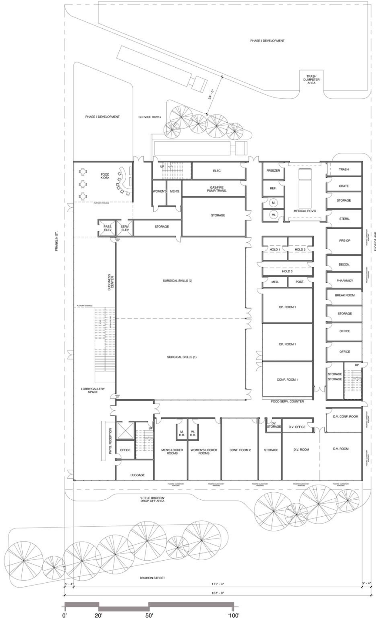
PROPOSED SCHEME I - GROUND PLAN NOT TO SCALE
